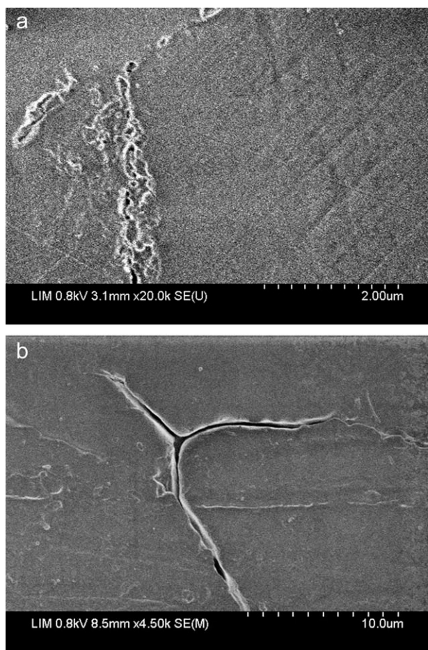
Figure 3 SEM observation of the most constrained area of a specimen tested at 10 Hz and \epsilon = 0.013 (interrupted test), (a) after 300,000 loading cycles and (b) after 500,000 loading cycles.
