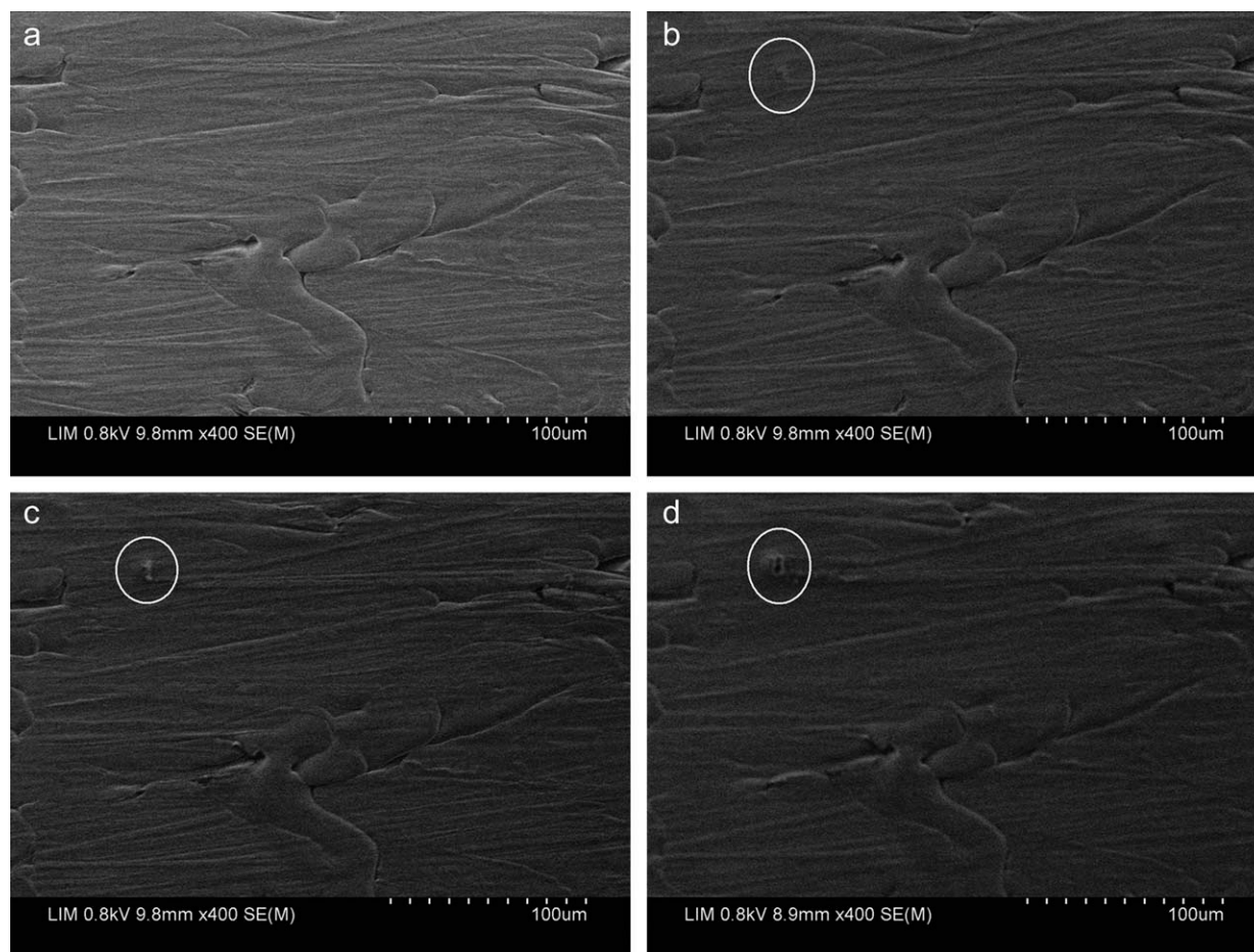
Figure 7 SEM observation of the most constrained and polished area of a specimen tested at 10 Hz and \epsilon = 0.017 (poly-sequential test) (a): initial, (b) 1000 cycles, T = 35^\circ\text{C} , (c) 5,000 cycles, T = 52^\circ\text{C} , (d) 10,000 cycles, T = 55^\circ\text{C} . The white circles indicate the fiber ends that are pulled out.
