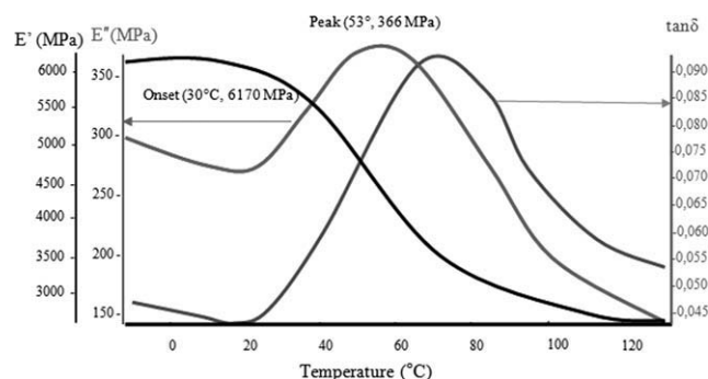
Figure 5 Viscoelastic spectrum of PA66/glass fiber at 10 Hz between -10 and 130°C.
