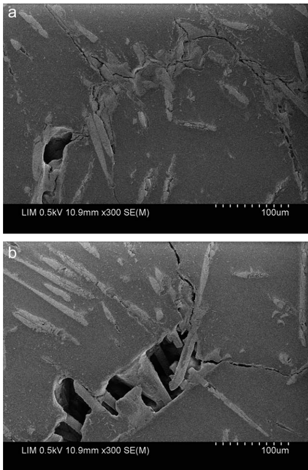
Figure 8 SEM observation of the most constrained and unpolished area of a specimen tested at 10 Hz, just before fracture (62,000 cycles). (a) Crack propagation in zones with a high fibers concentration and (b) crack propagation in the matrix.
