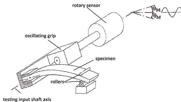
Figure 2 Alternative bending device used for fatigue tests. 6
