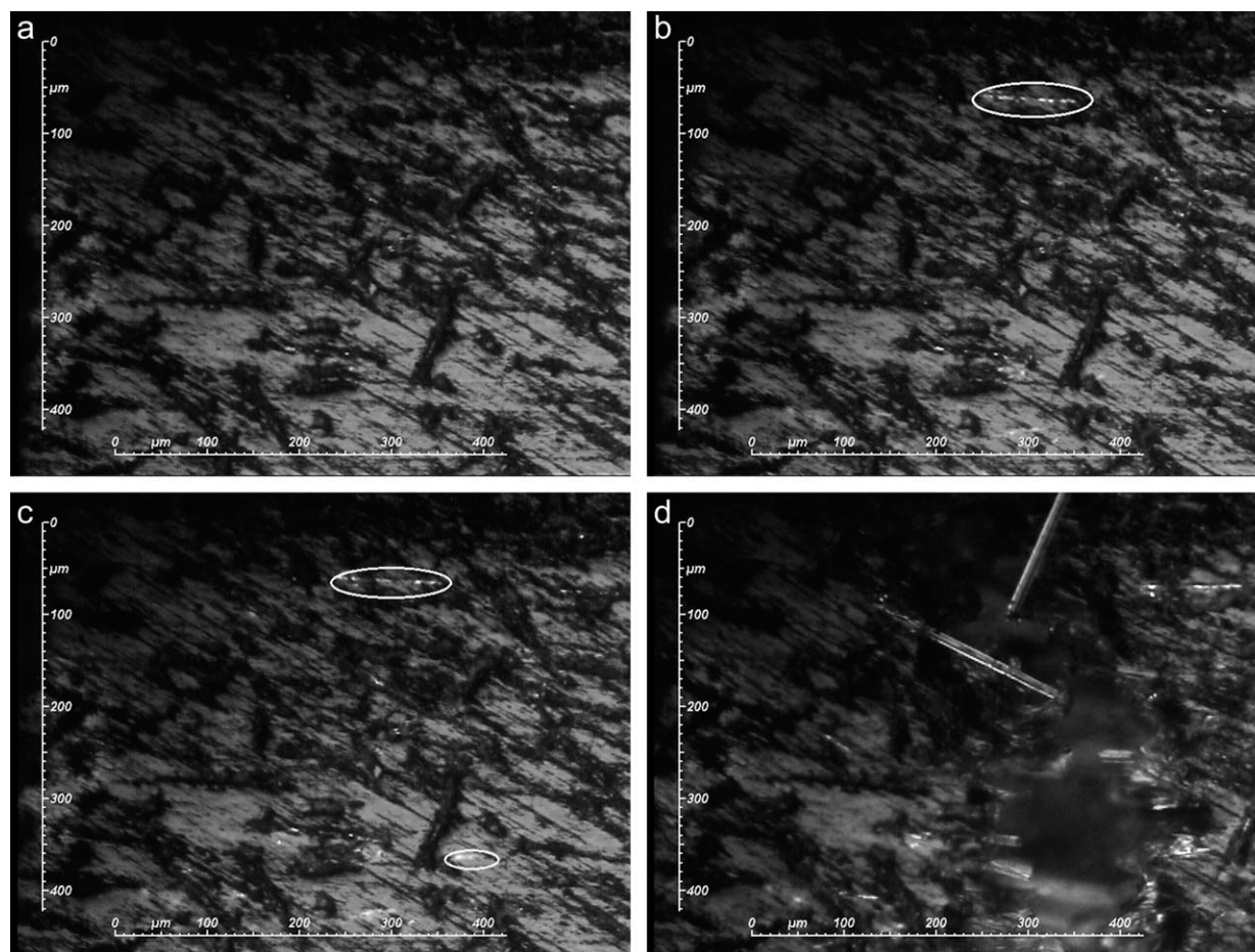
Figure 6 Optical microscopy observation of the most constrained part of a specimen tested at 10 Hz and \varepsilon = 0.017 (poly-sequential test) (a) initial, (b) 30,000 cycles, T = 57^\circ\text{C} , (c) 45,000 cycles, T = 60^\circ\text{C} , (d) 60,000 cycles, T = 62^\circ\text{C} .
